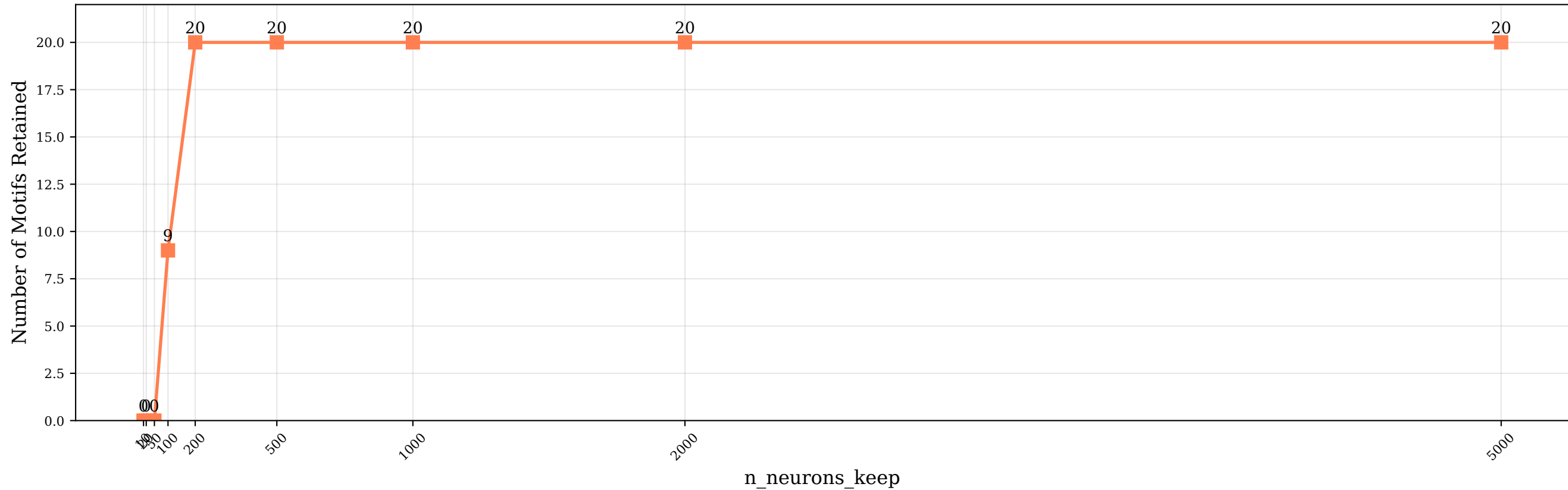
Motif Retention vs Neuron Threshold sigma: (1, 1) | volume: (0.03, 0.9)
